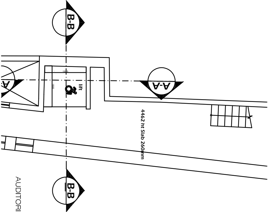
Part Plan SF SCALE 1:100
