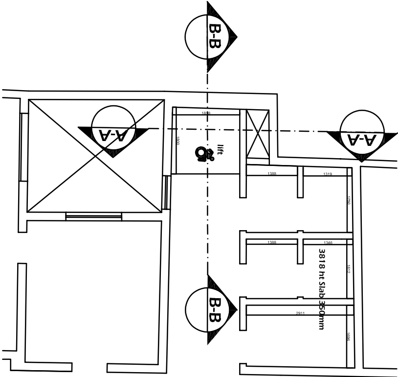
Part Plan GF SCALE 1:100
